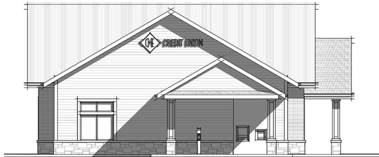
drive-up elevation
